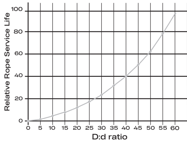
Service life curve for various D:d ratios
