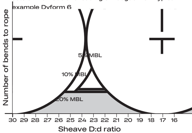
Effects of D:d Ratio and loading on fatigue life - Typical
